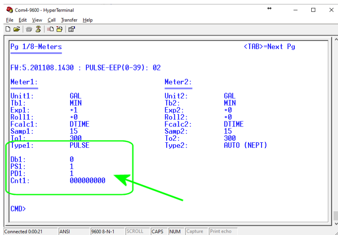
Figure 9B. Serial Terminal / Telnnet Pulse Setup Screen
