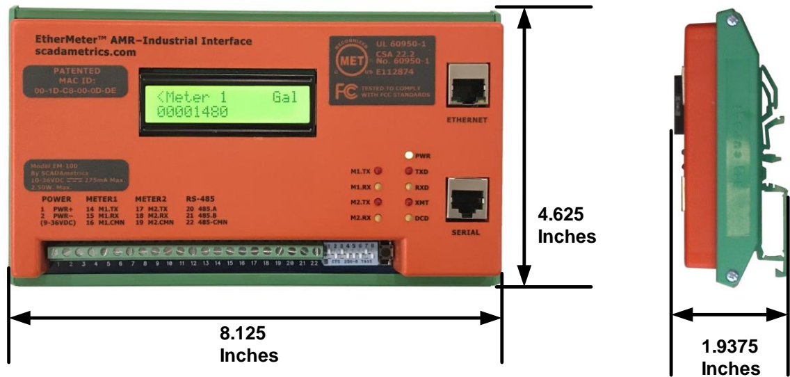
Figure 3A. Dimensional Drawing
