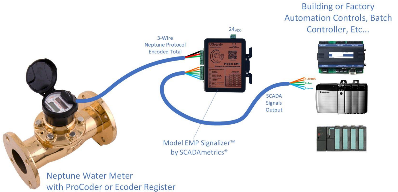
Neptune Water Meter with Signalizer.
