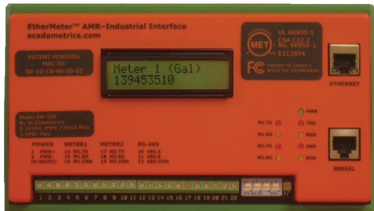
EtherMeter™ SCADA/Meter Gateway By SCADAmetrics
