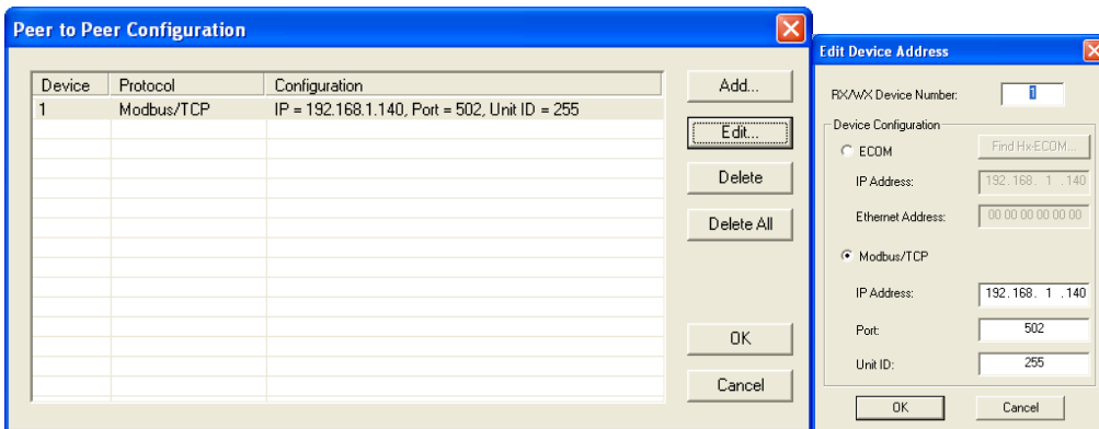
Figure 9. Ethernet Port Configuration Dialog Boxes
